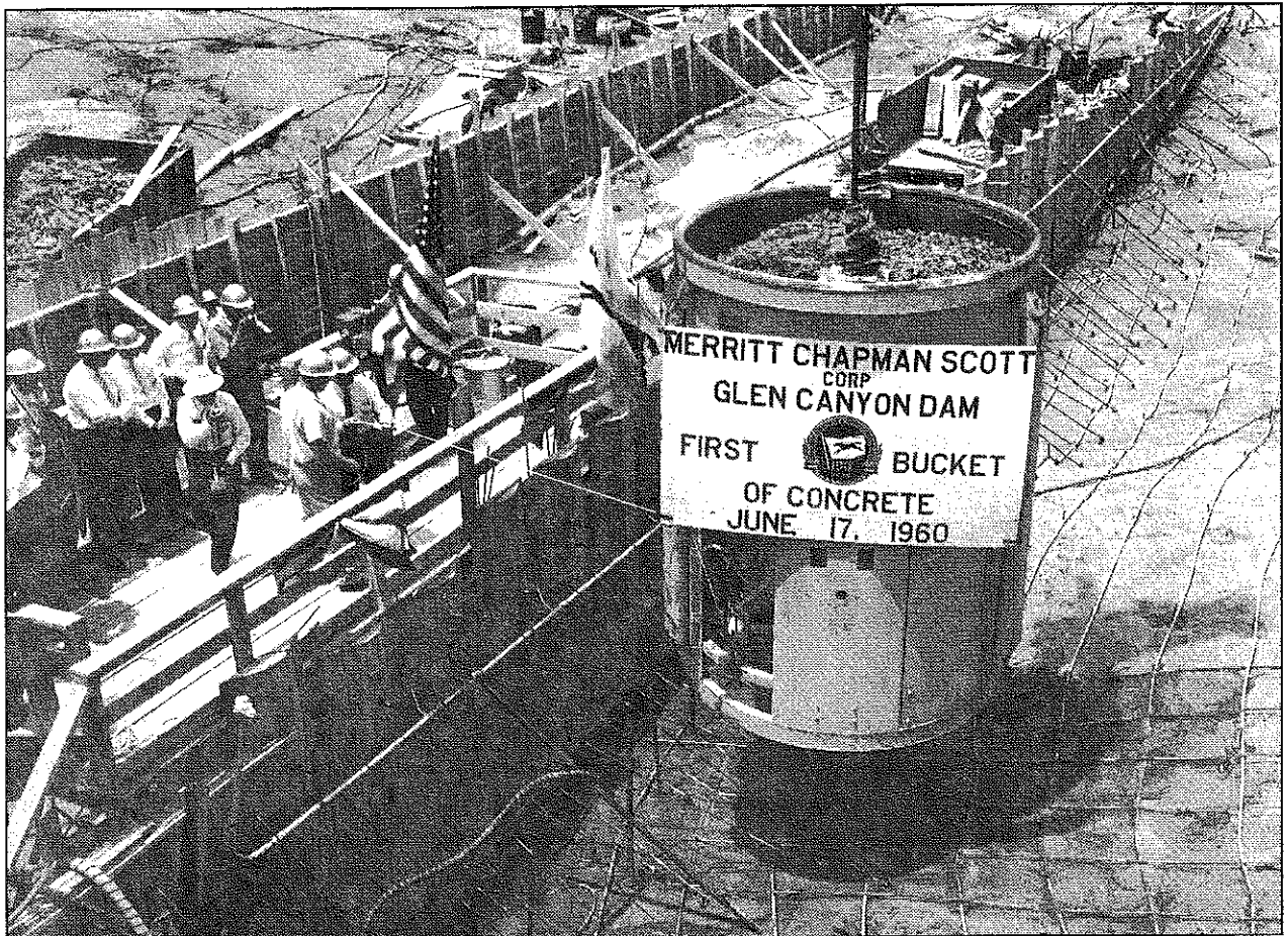
First bucket of concrete being added to the Glen Canyon Dam, 1960. John Wesley Powell Museum.
